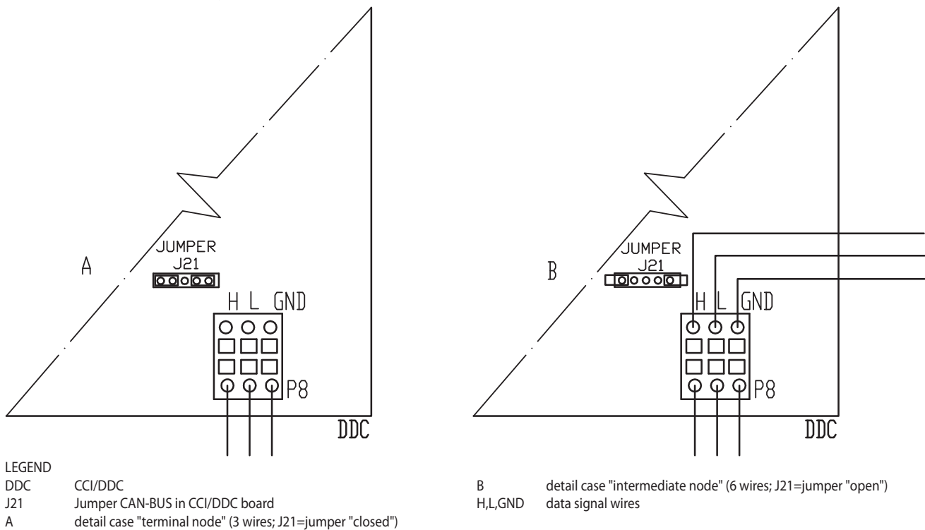
Figure 5.16 – detail wires and jumpers J21 - terminal/intermediate node CCI/DDC
