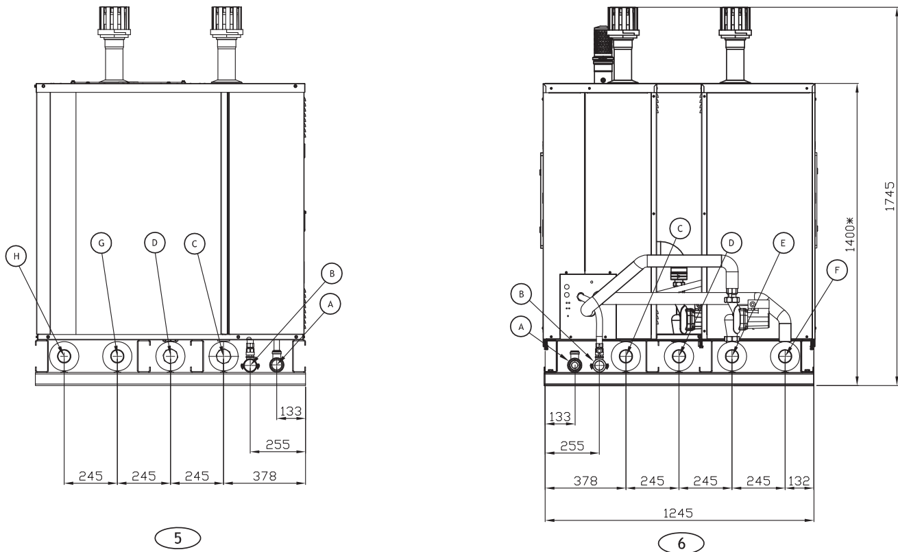
Figure 2.11 – Water, gas and condensate discharge fittings position, for groups a 6 pipes
