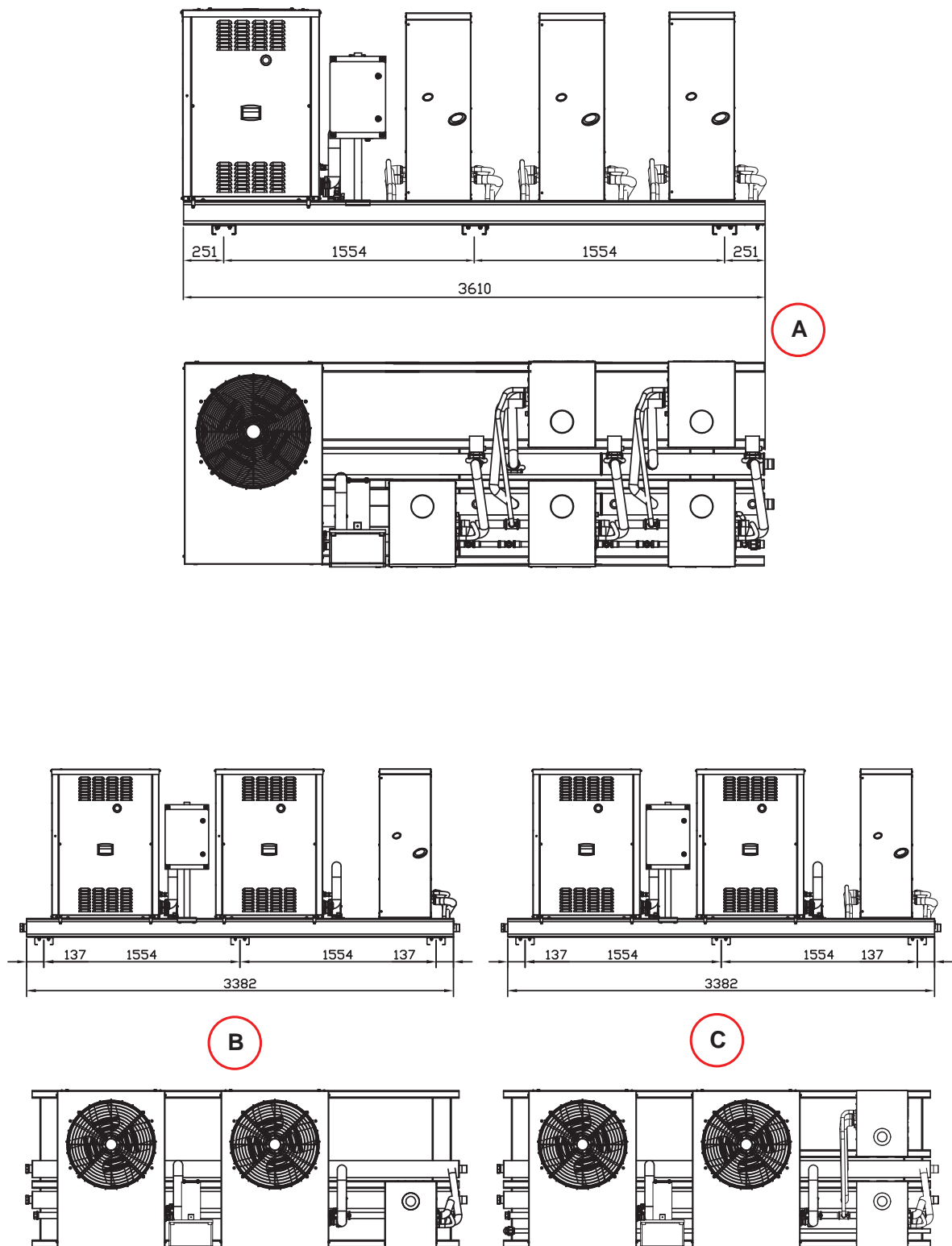
Figure 2.16 – Preassembled ACF/A/AR + AY group (with 1+5, 2+1 and 2+2 units)
