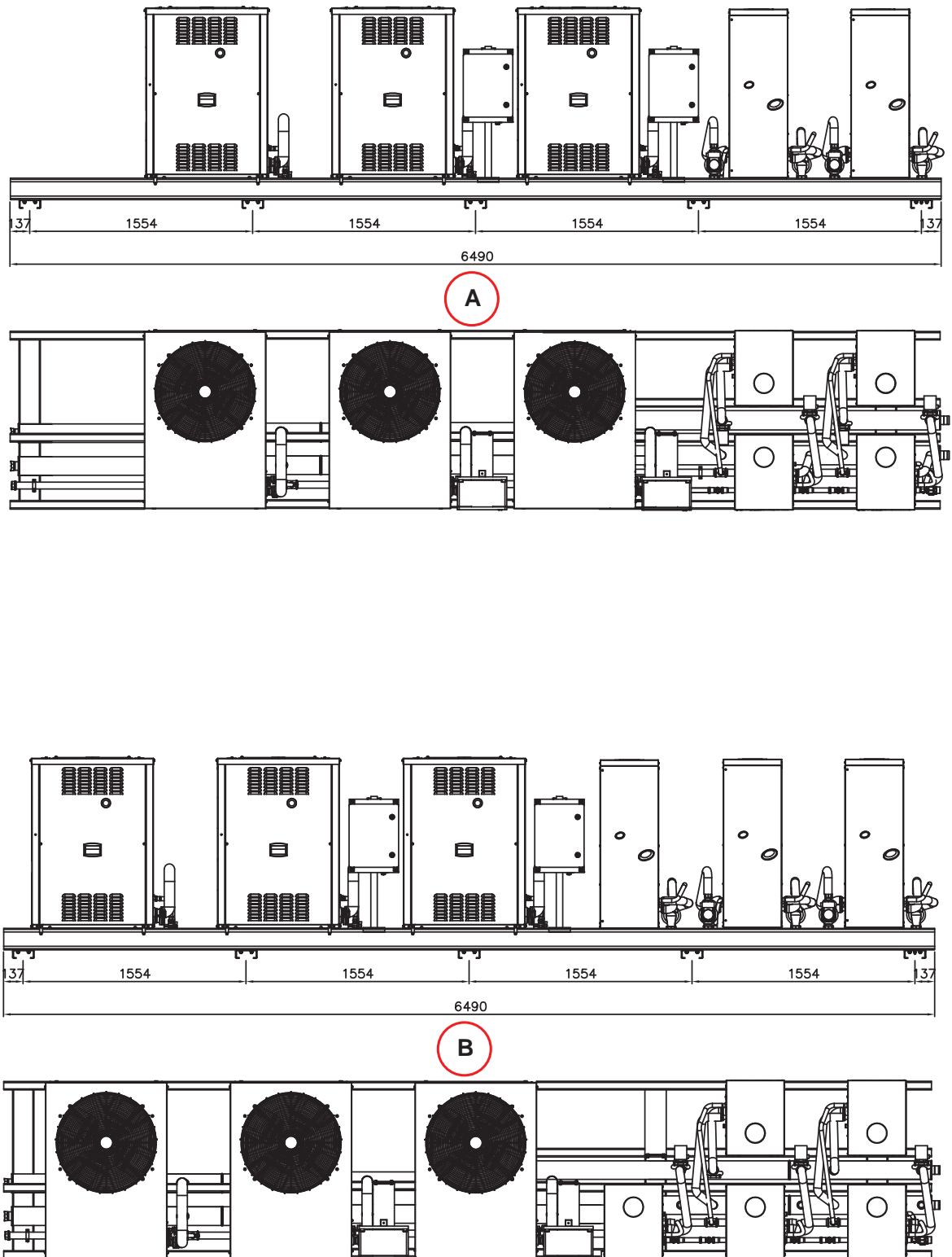
Figure 2.20 – Preassembled ACF/A/AR + AY group (with 3+4 and 3+5 units)
