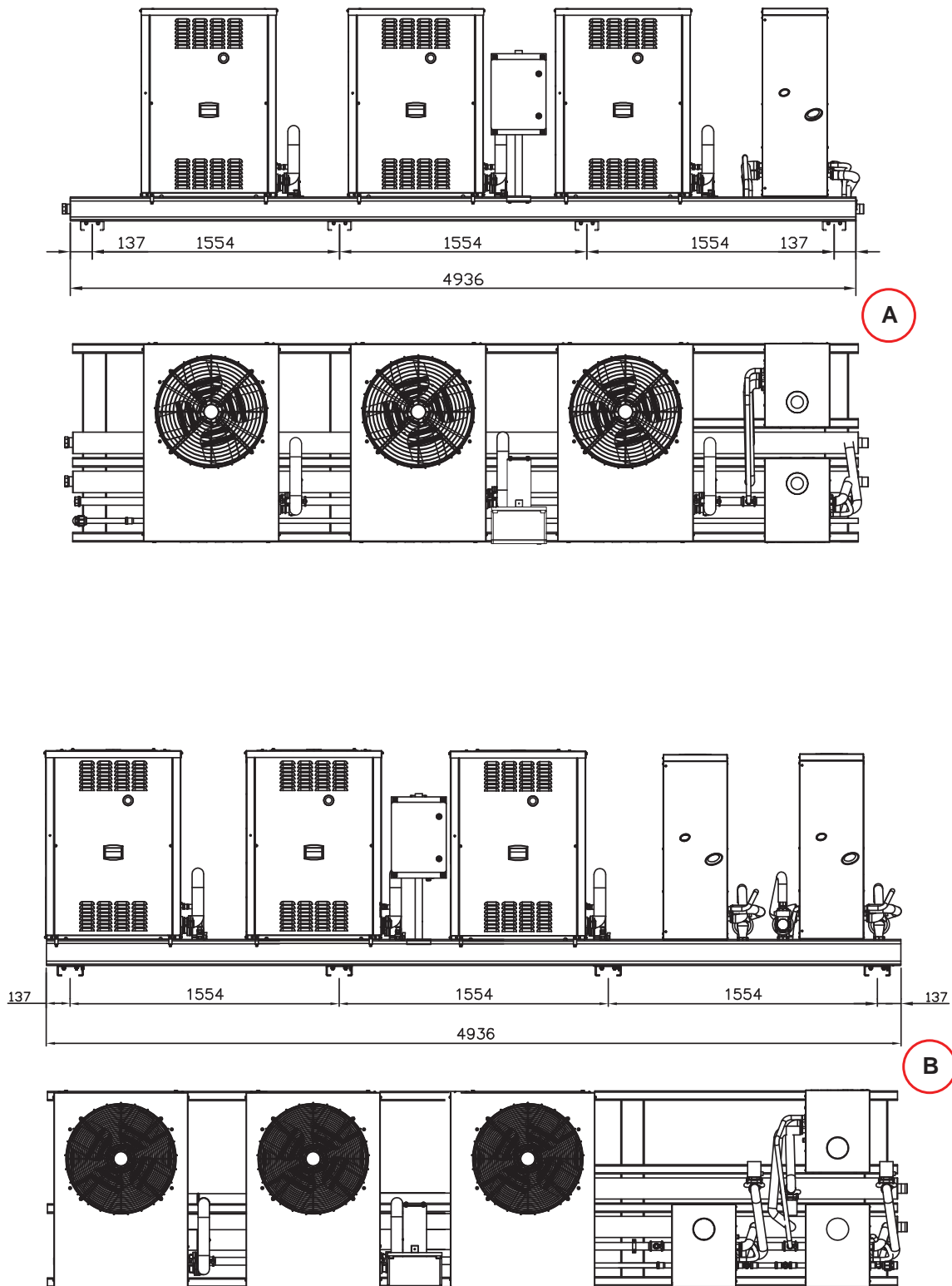
Figure 2.19 – Preassembled ACF/A/AR + AY group (with 3+2 and 3+3 units)
