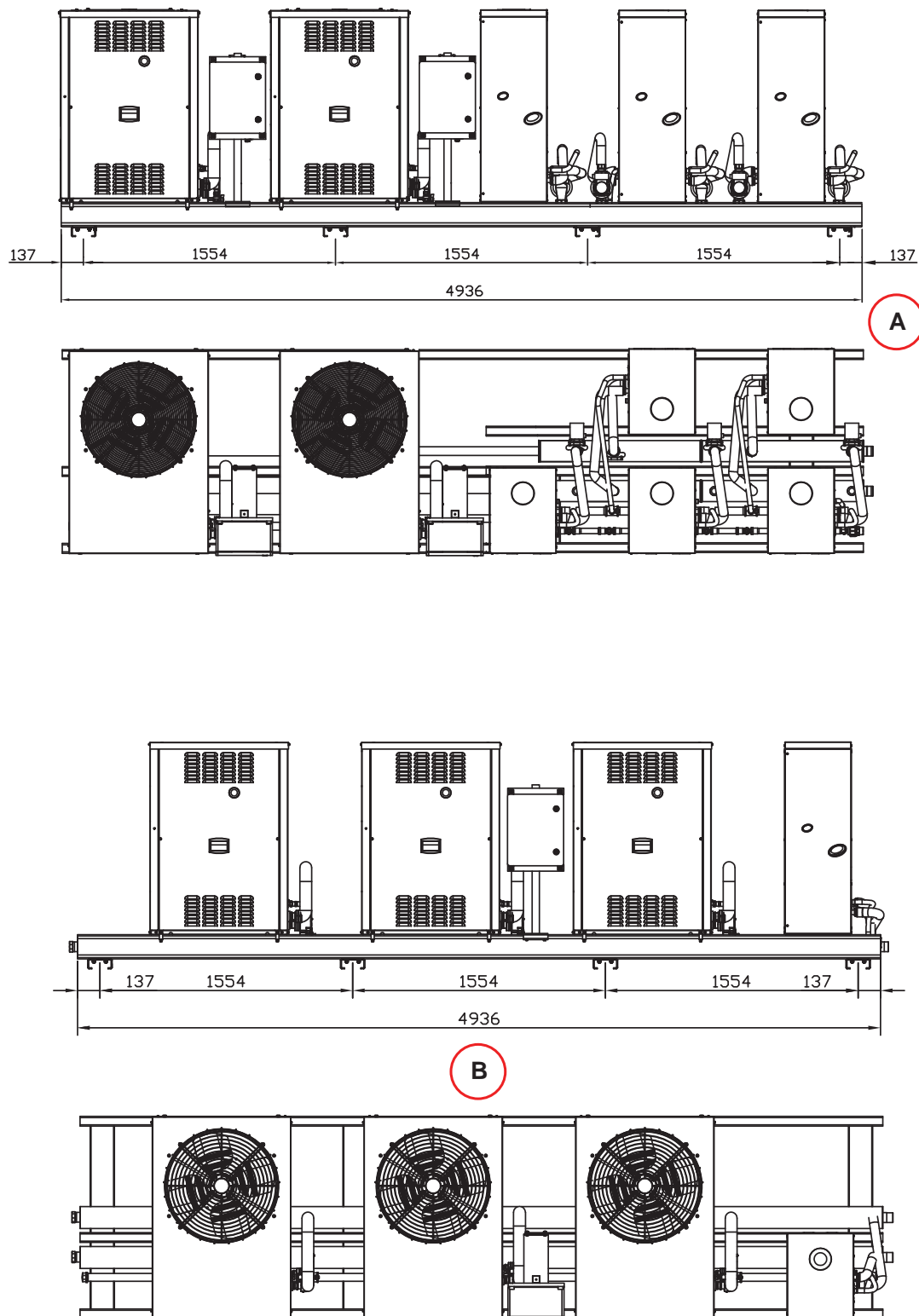
Figure 2.18 – Preassembled ACF/A/AR + AY group (with 2+5 and 3+1 units)
