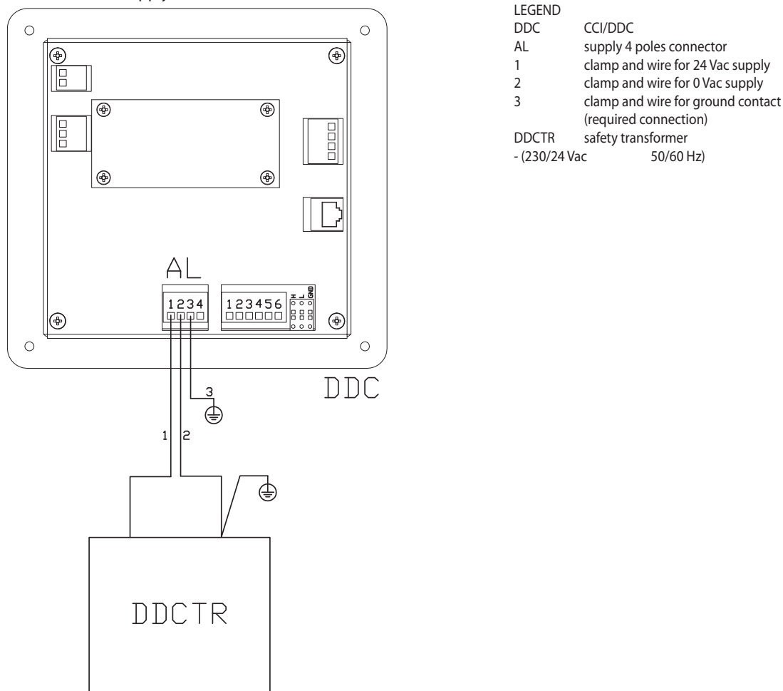
Figure 5.11 – CCI/DDC - electric supply
