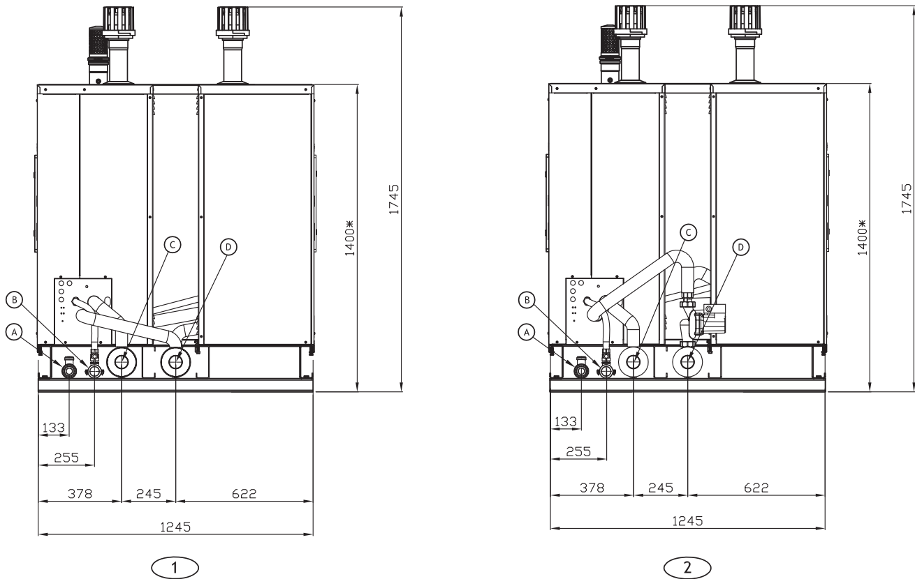
Figure 2.9 – Water, gas and condensate discharge fittings position, for groups a 2 pipes
