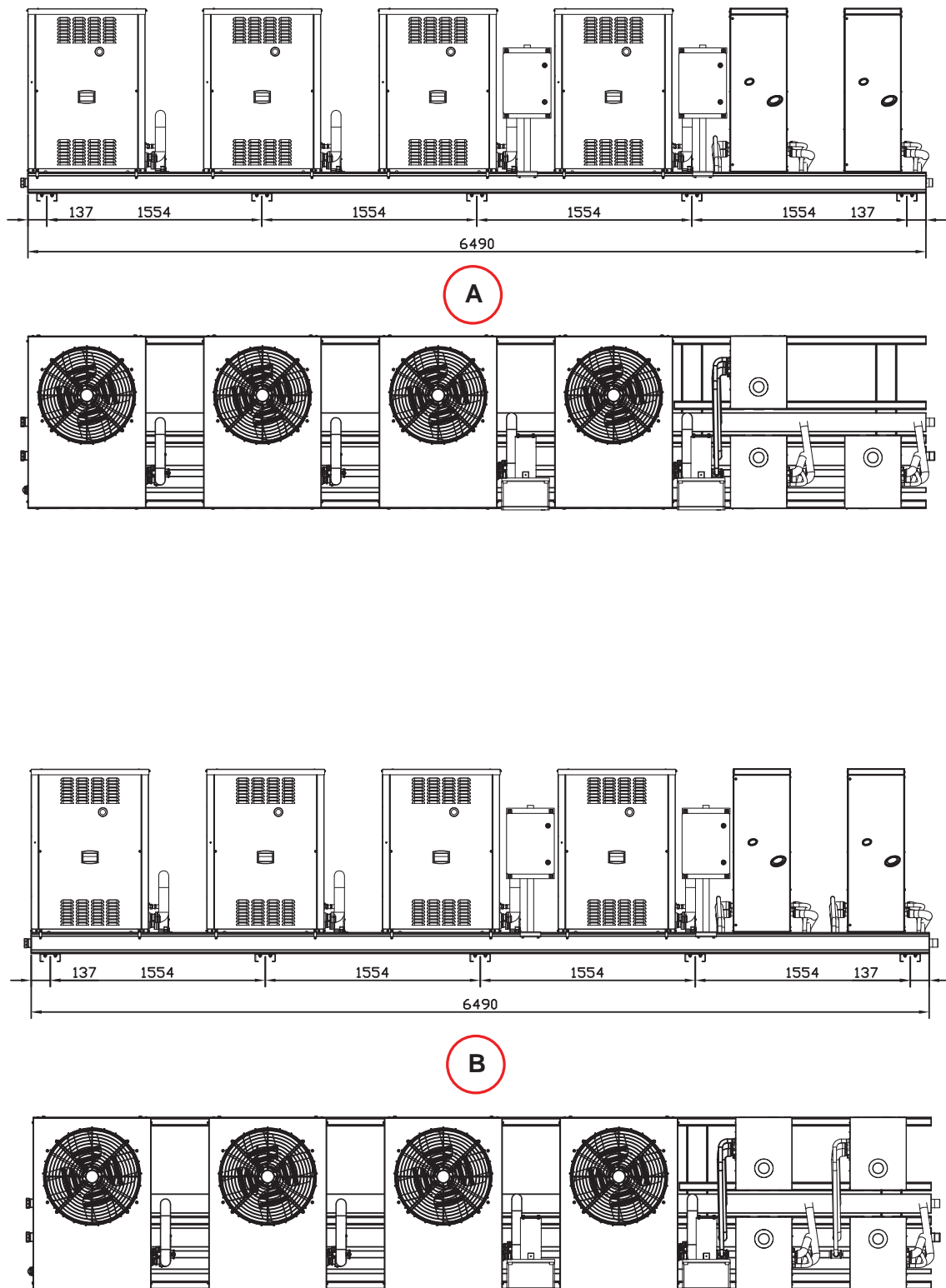
Figure 2.22 – Preassembled ACF/A/AR + AY group (with 4+3 and 4+4 units)
