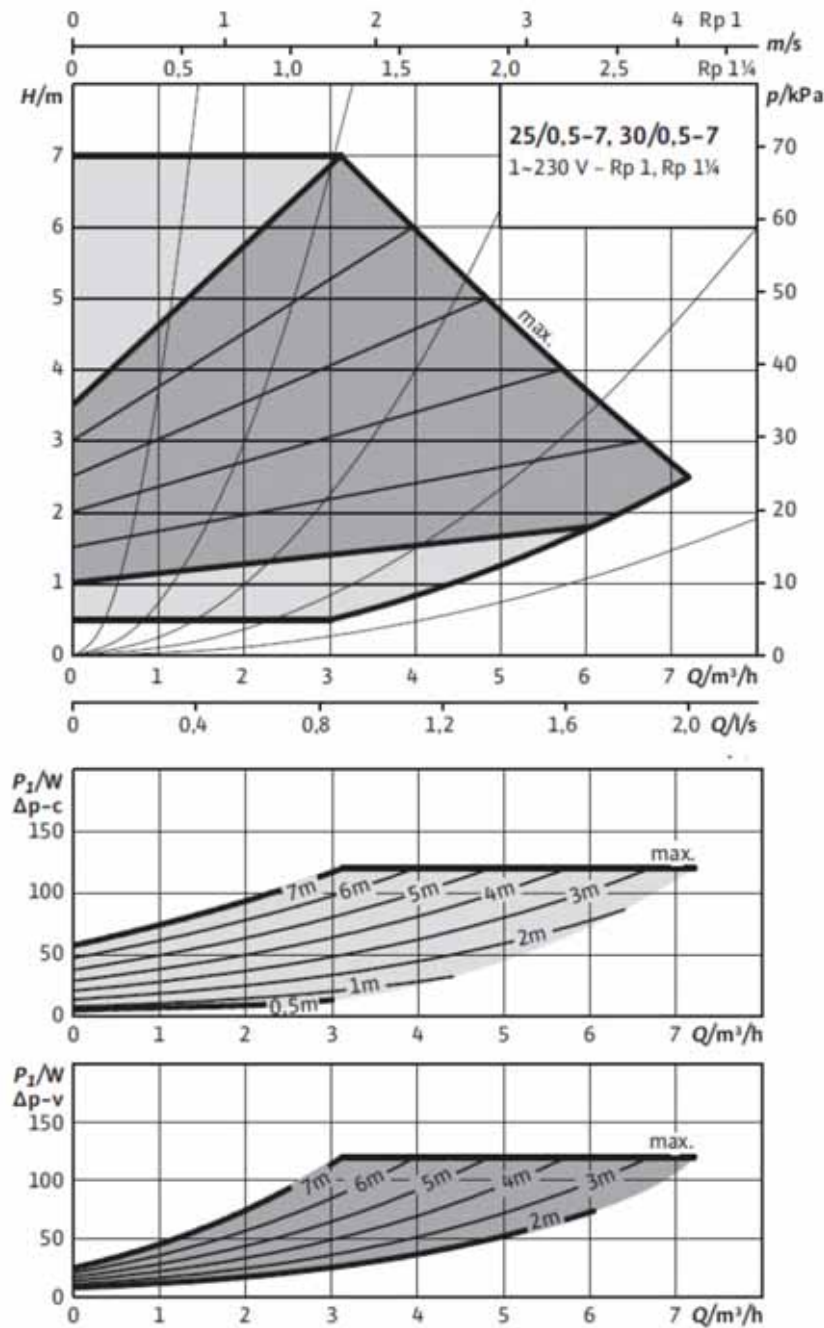
Figure 2.3 – Characteristic diagrams of WILO YONOS HF 25/7 pump
