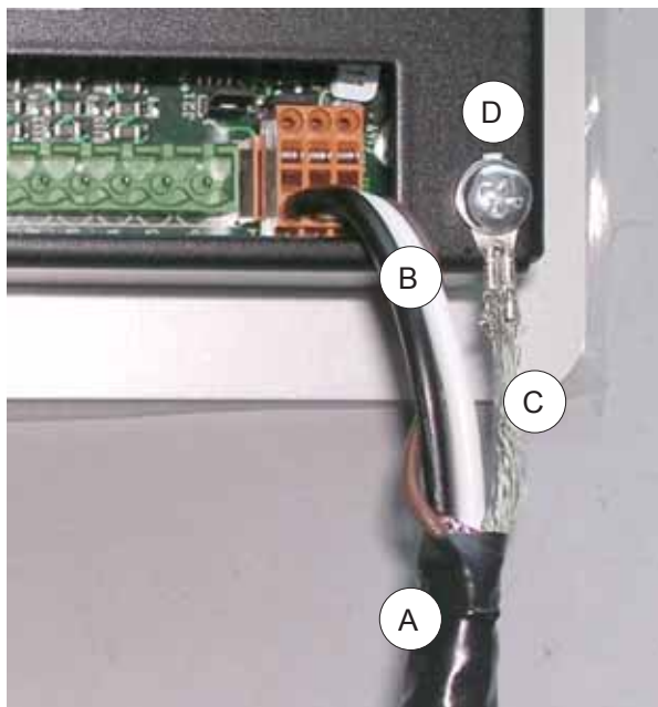
Figure 5.15 – Connection from CAN BUS to connector P8
