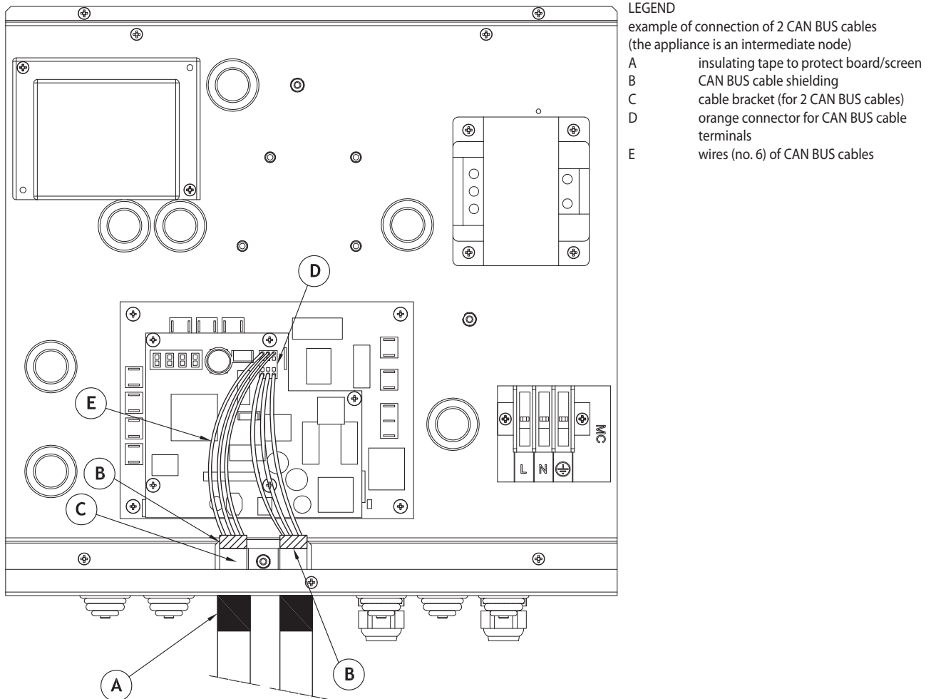
Figure 5.21 – Connection of CAN BUS cable to connector P8 on controller AY10
