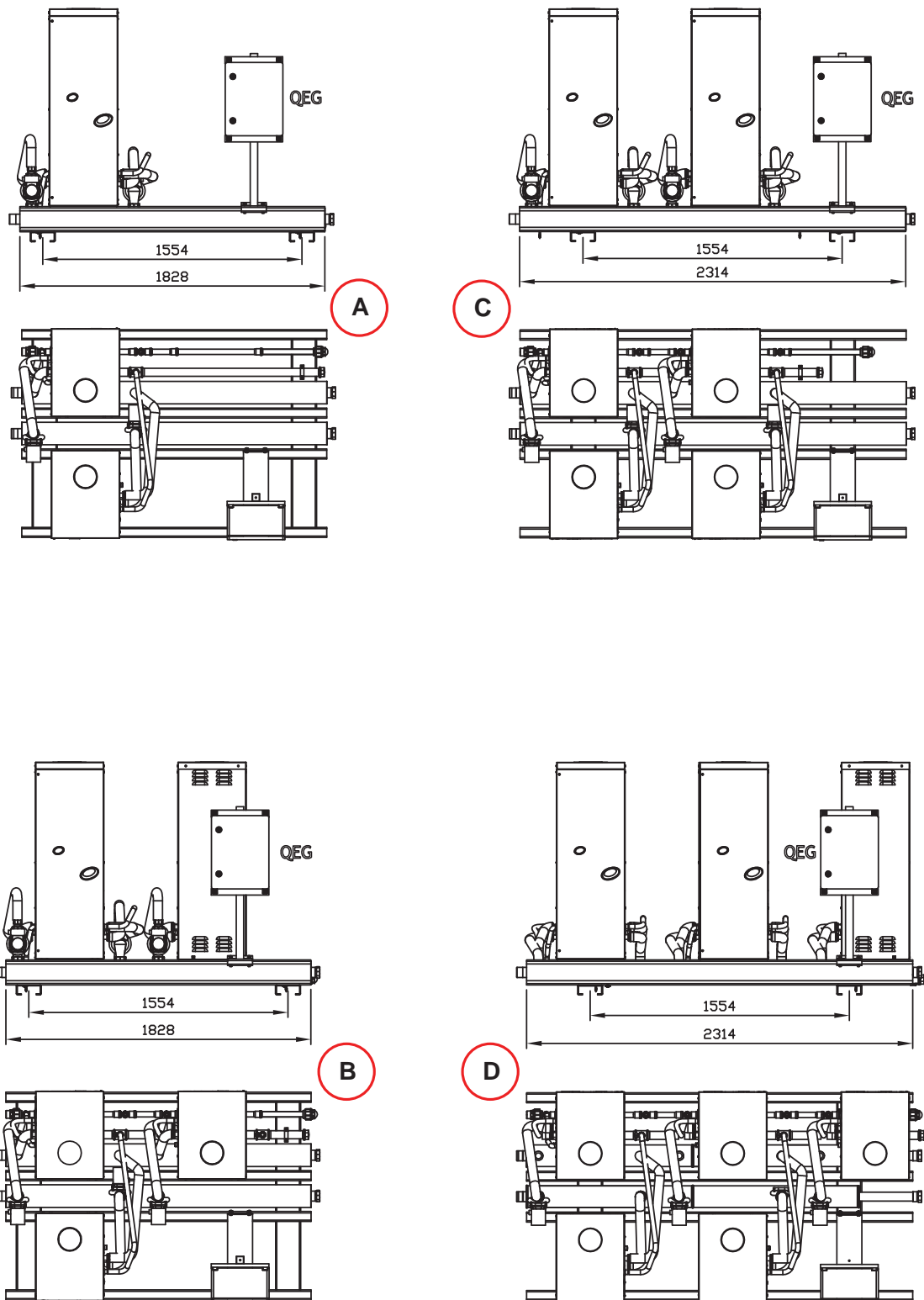
Figure 2.14 – Preassembled AY group (with 2, 3, 4 and 5 units)
