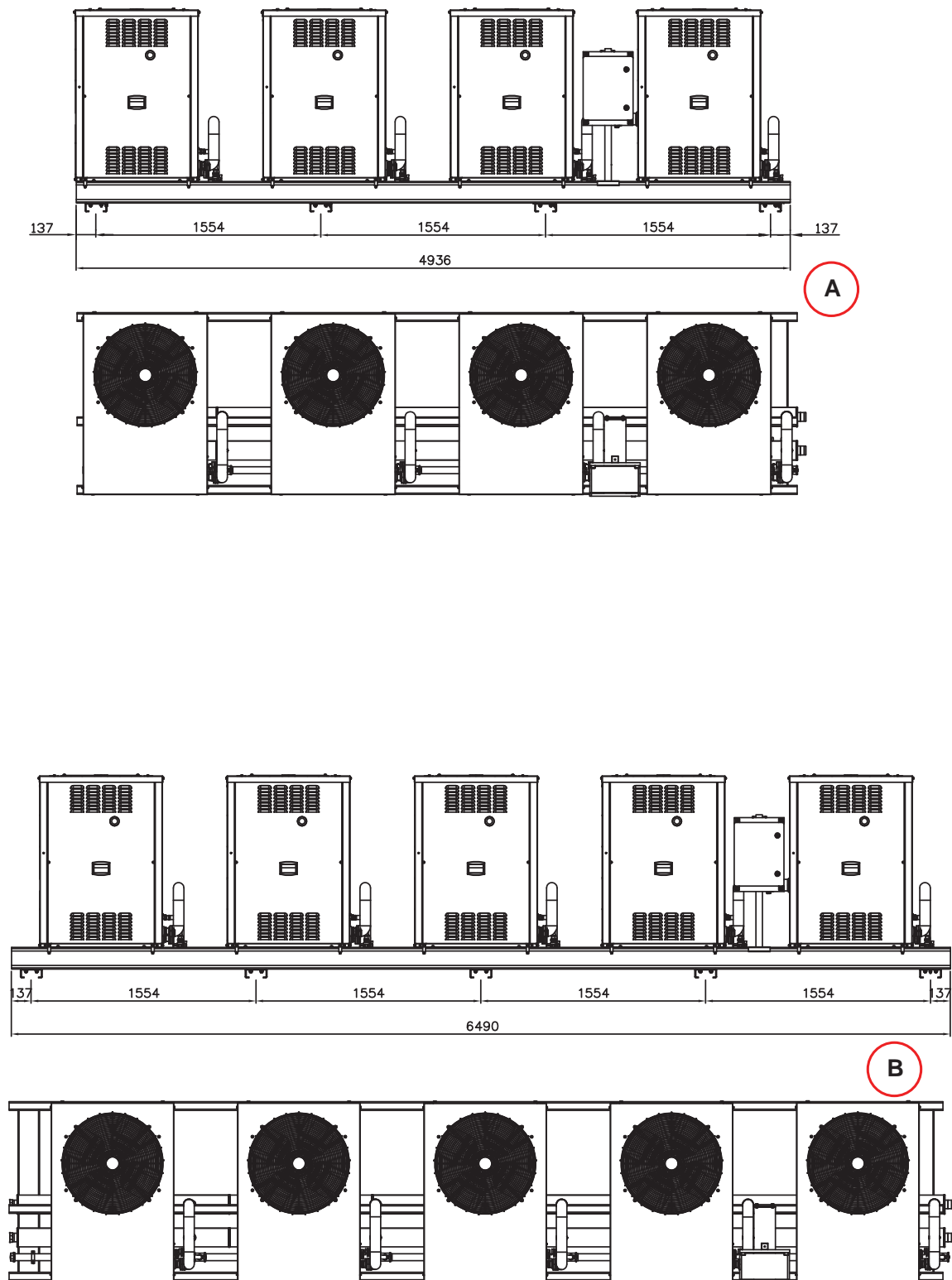
Figure 2.13 – Preassembled ACF/A/AR group (with 4 and 5 units)
