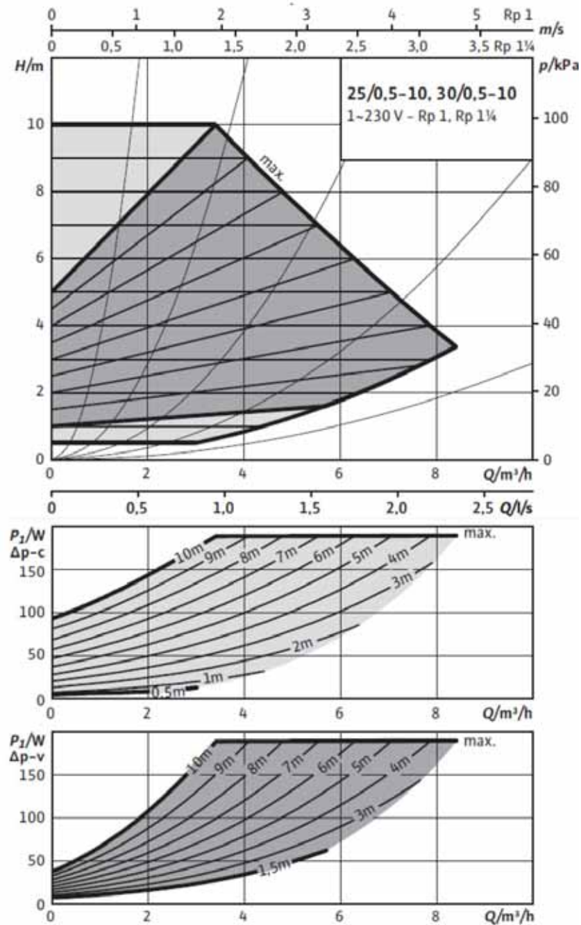
Figure 2.4 – Characteristic diagrams of WILO YONOS HF 25/10 pump
