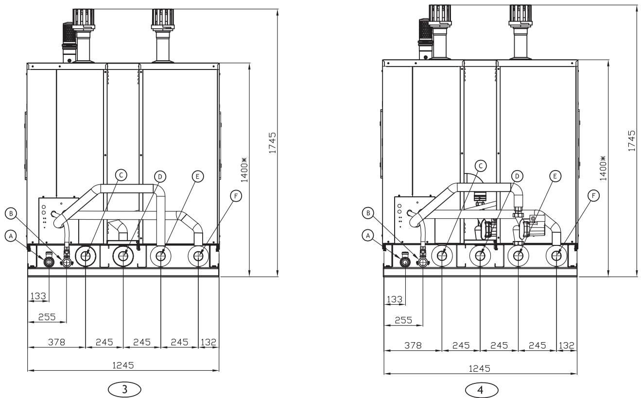
Figure 2.10 – Water, gas and condensate discharge fittings position, for groups a 4 pipes
