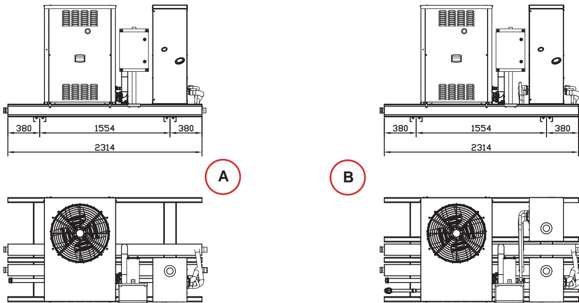
Figure 2.15 – Preassembled ACF or A or AR + AY group (with 1+1, 1+2, 1+3 and 1+4 units)
