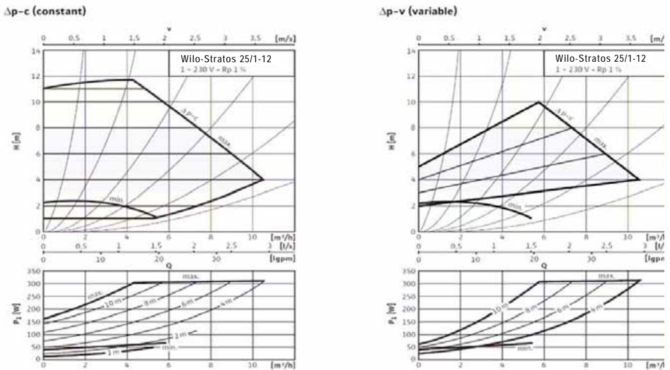
Figure 2.6 – Characteristic curves of WILO Stratos Para 25/1-12 pump
