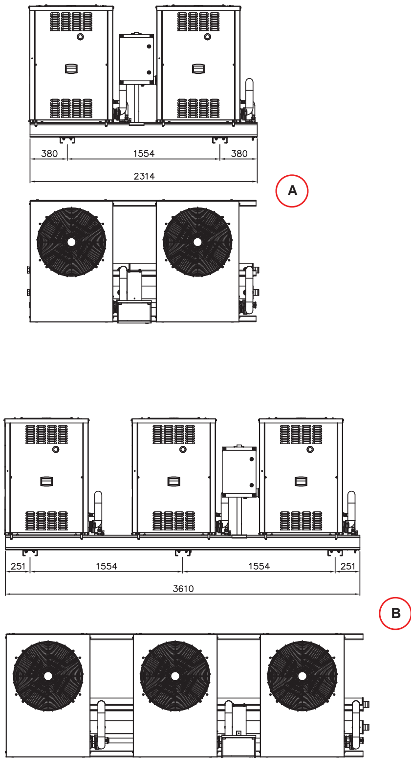
Figure 2.12 – Preassembled ACF/A/AR group (with 2 and 3 units)
