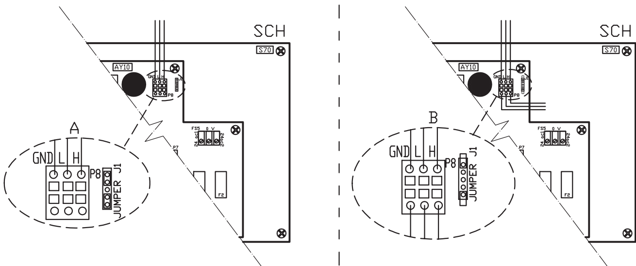
Figure 5.22 – detail of wires and jumpers J1 - appliance terminal/intermediate node
